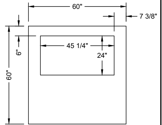
SLAB DETAIL - 24" x 45 1/4" ACCESS
