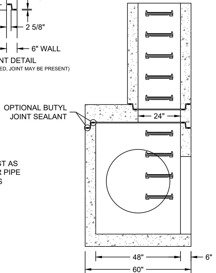
SECTION B-B
