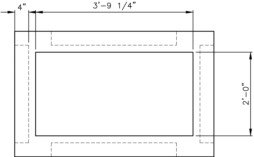
PLAN VIEW SCALE: 3/4" = 1'-0"
