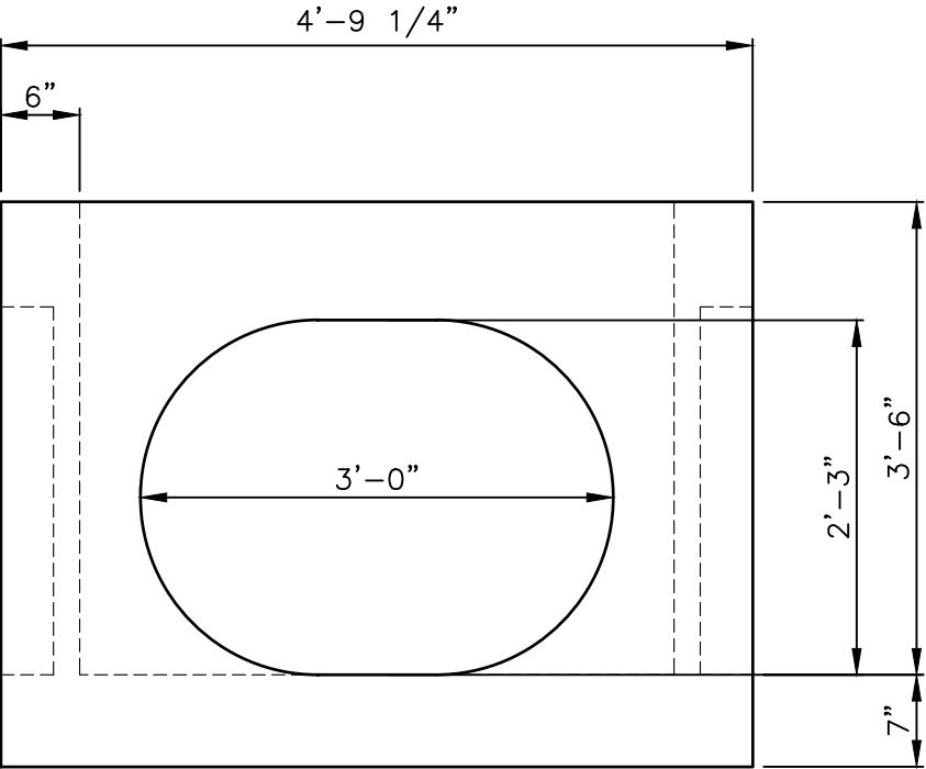
FRONT VIEW SCALE: 3/4" = 1'-0"
