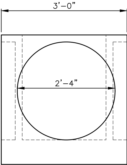
SIDE PROFILE SCALE: 3/4" = 1'-0"
