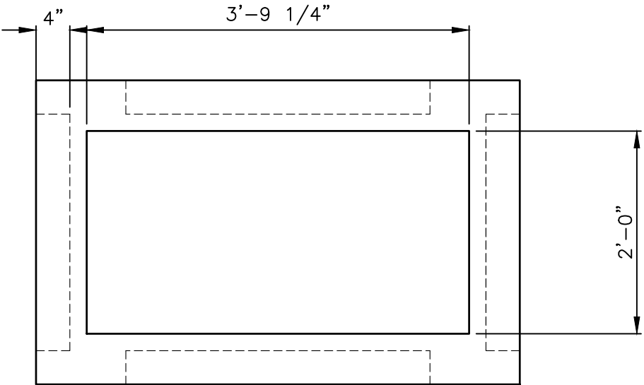
PLAN VIEW SCALE: 3/4" = 1'-0"
