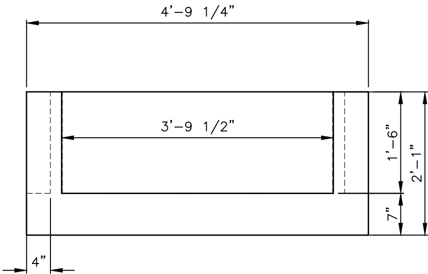
FRONT PROFILE
