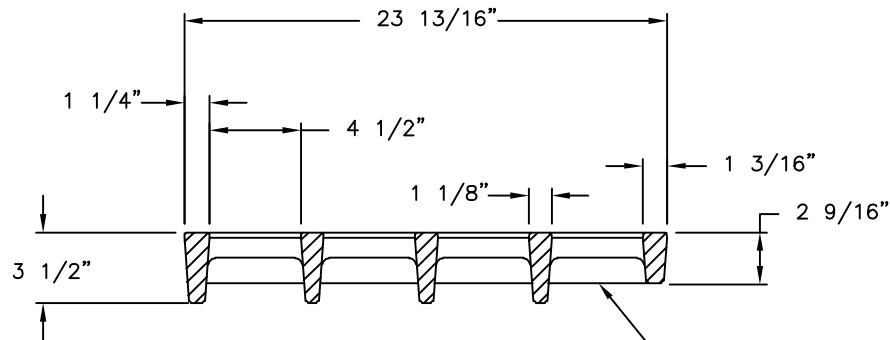
SECTION OF GRATE
