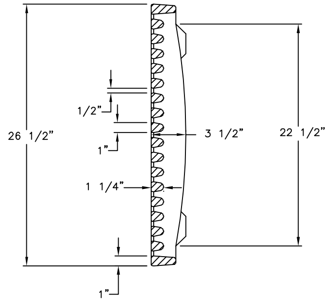
SECTION OF GRATE
