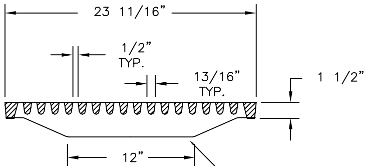
GRATE SECTION
