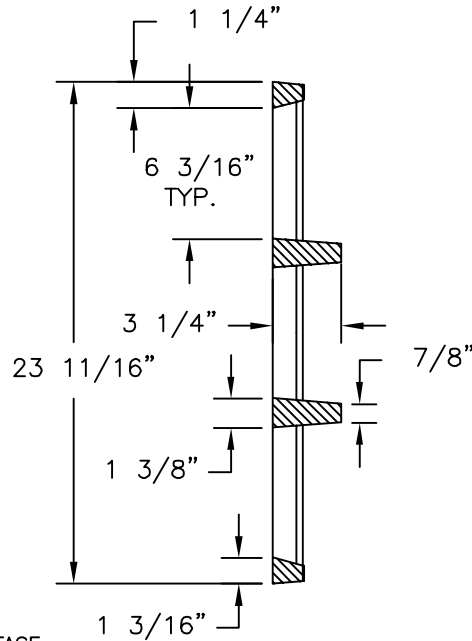
GRATE SECTION
