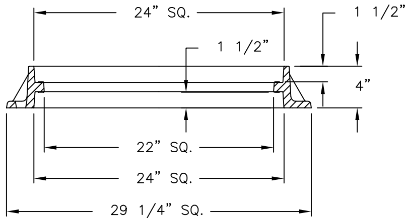
FRAME SECTION
