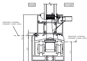
6a-6e - Threshold and Drainage Details
