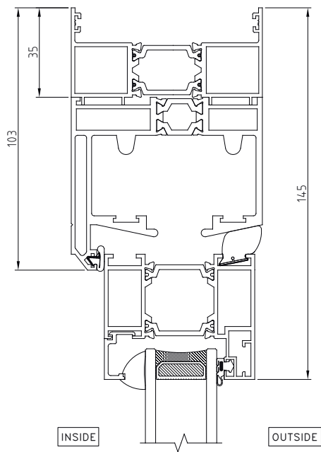
22b Bi-Fold Frame Extender With Trickle Vent Detail
