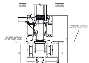
7a-7b - Non-Weathered Threshold Detail
