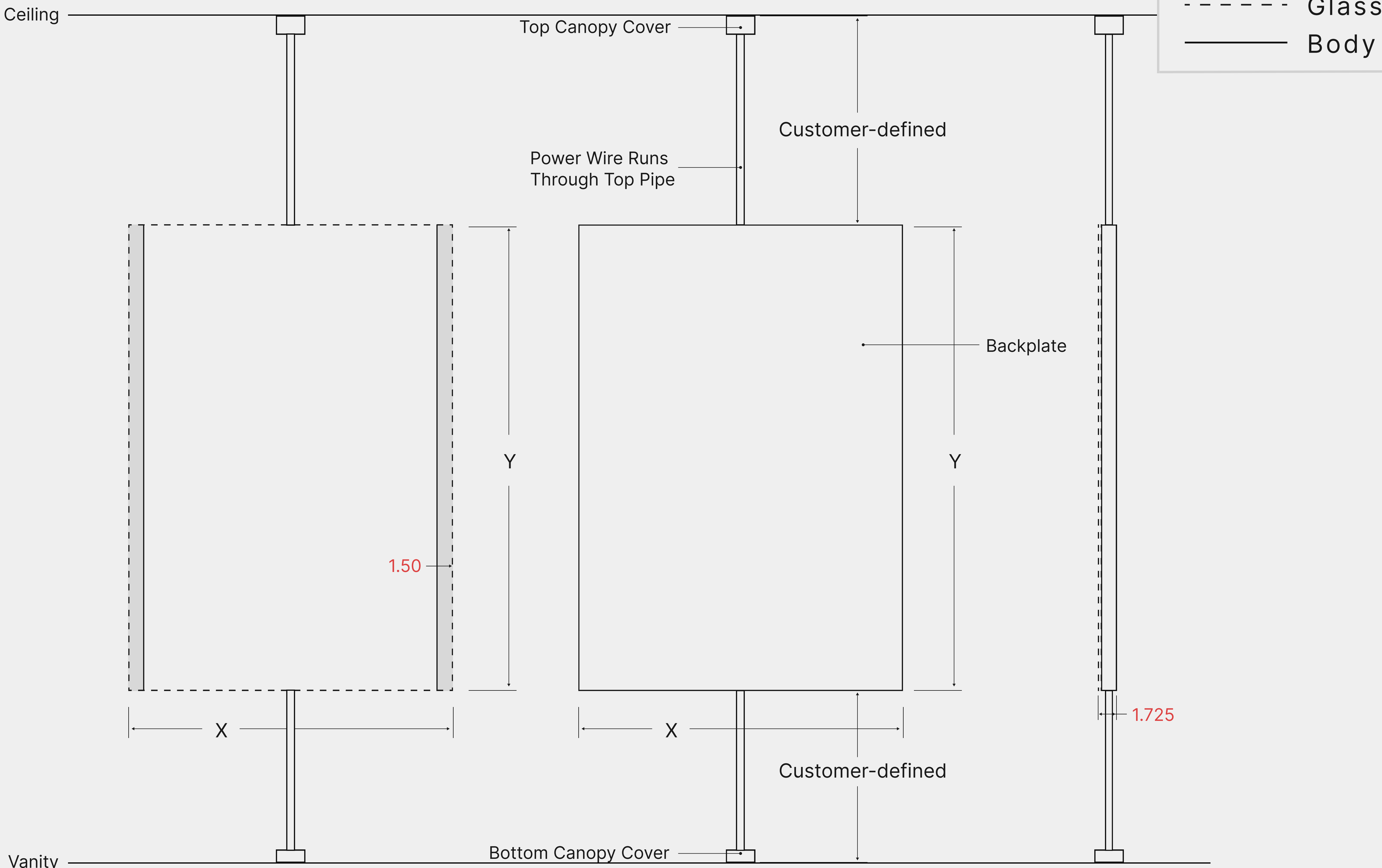
FRONT
