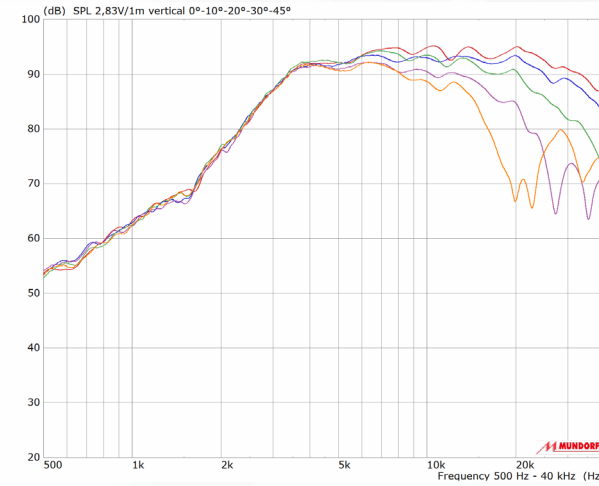
SPL Vertical 0° - 10° - 20° - 30° - 45°
