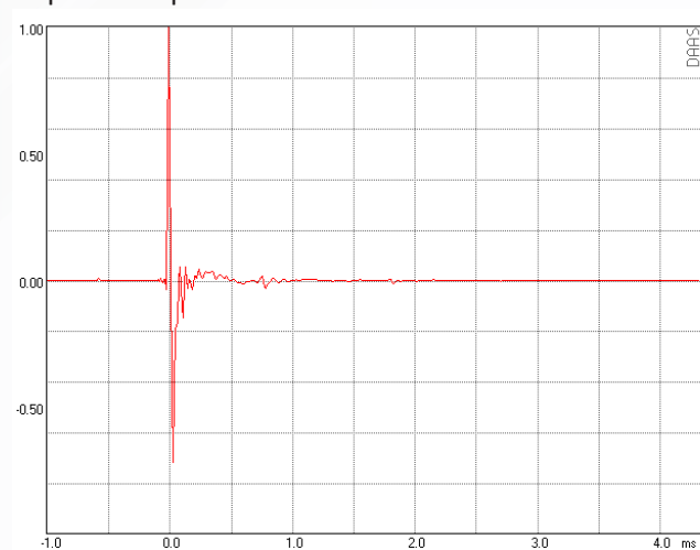
Impulse Response
