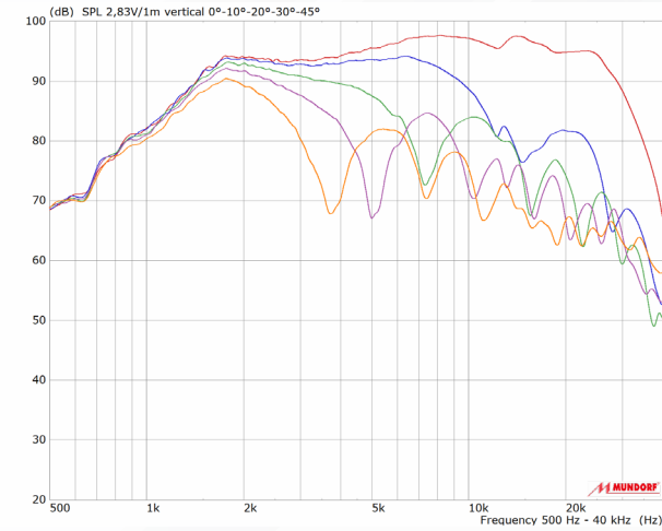
SPL Vertical 0° - 10° - 20° - 30° - 45°
