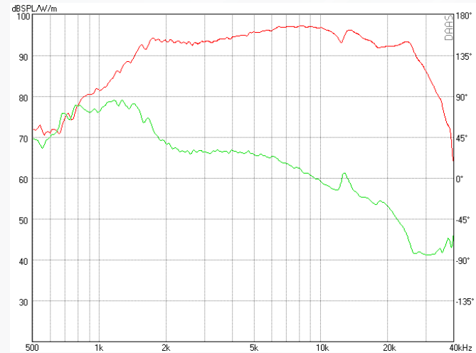
SPL - Phase
