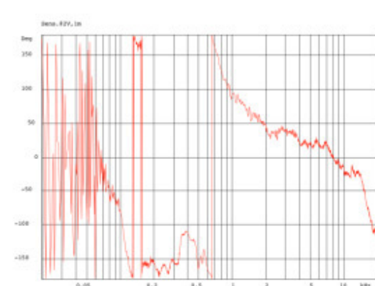
Figure 6: Tweeter phase
