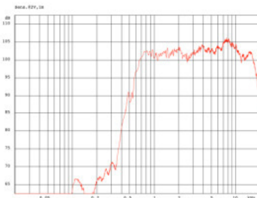
Figure 5: Frequency response of tweeter
