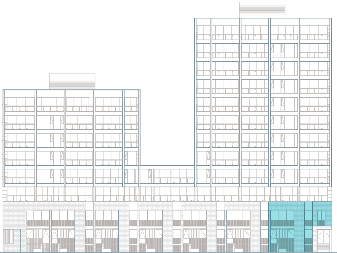
Northern Elevation - Boundary Road
