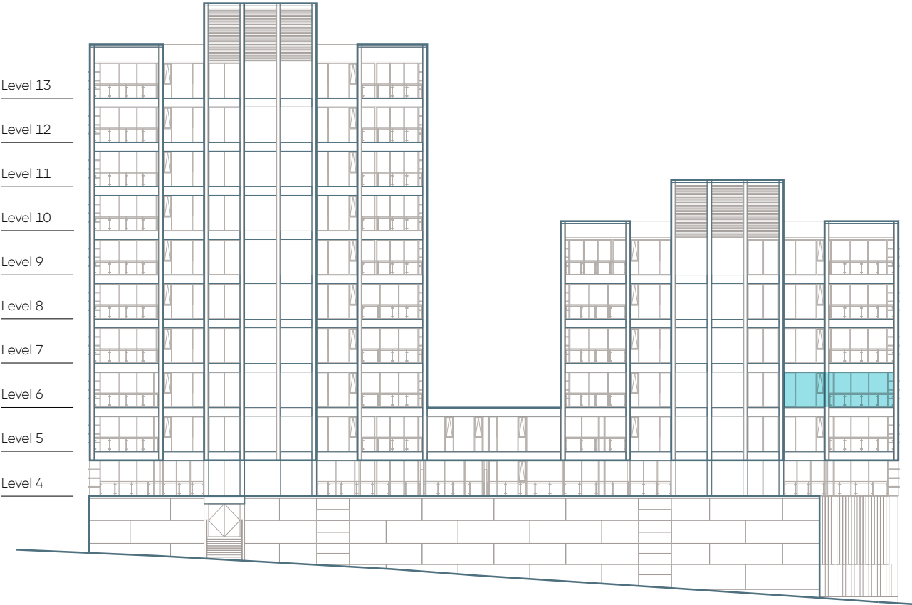
Southern Elevation - Launch Road
