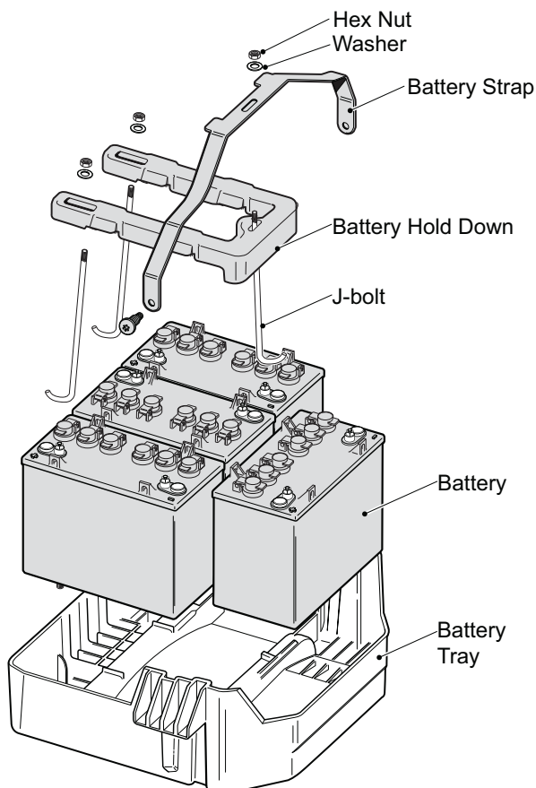
Fig. 28 Battery Components
