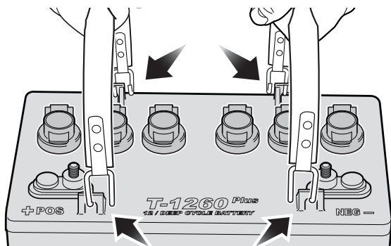
Fig. 26 Battery Removal
