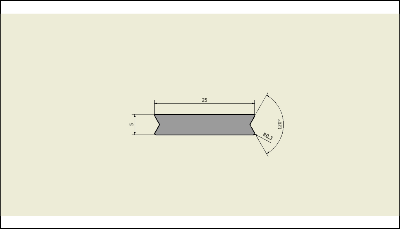
Fishtail 25.0 x 5.0
