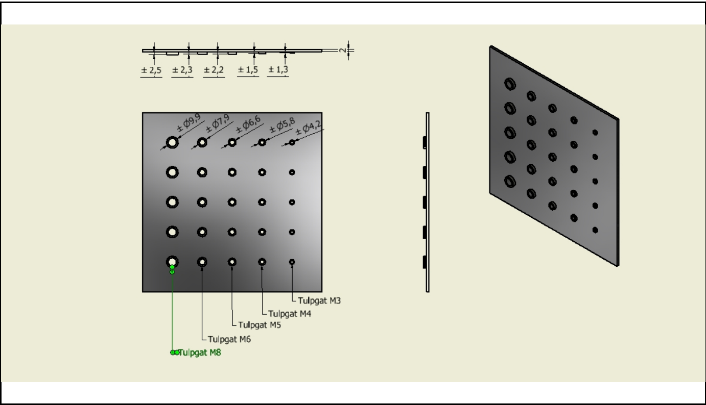
Tulpgat M6 downwards
