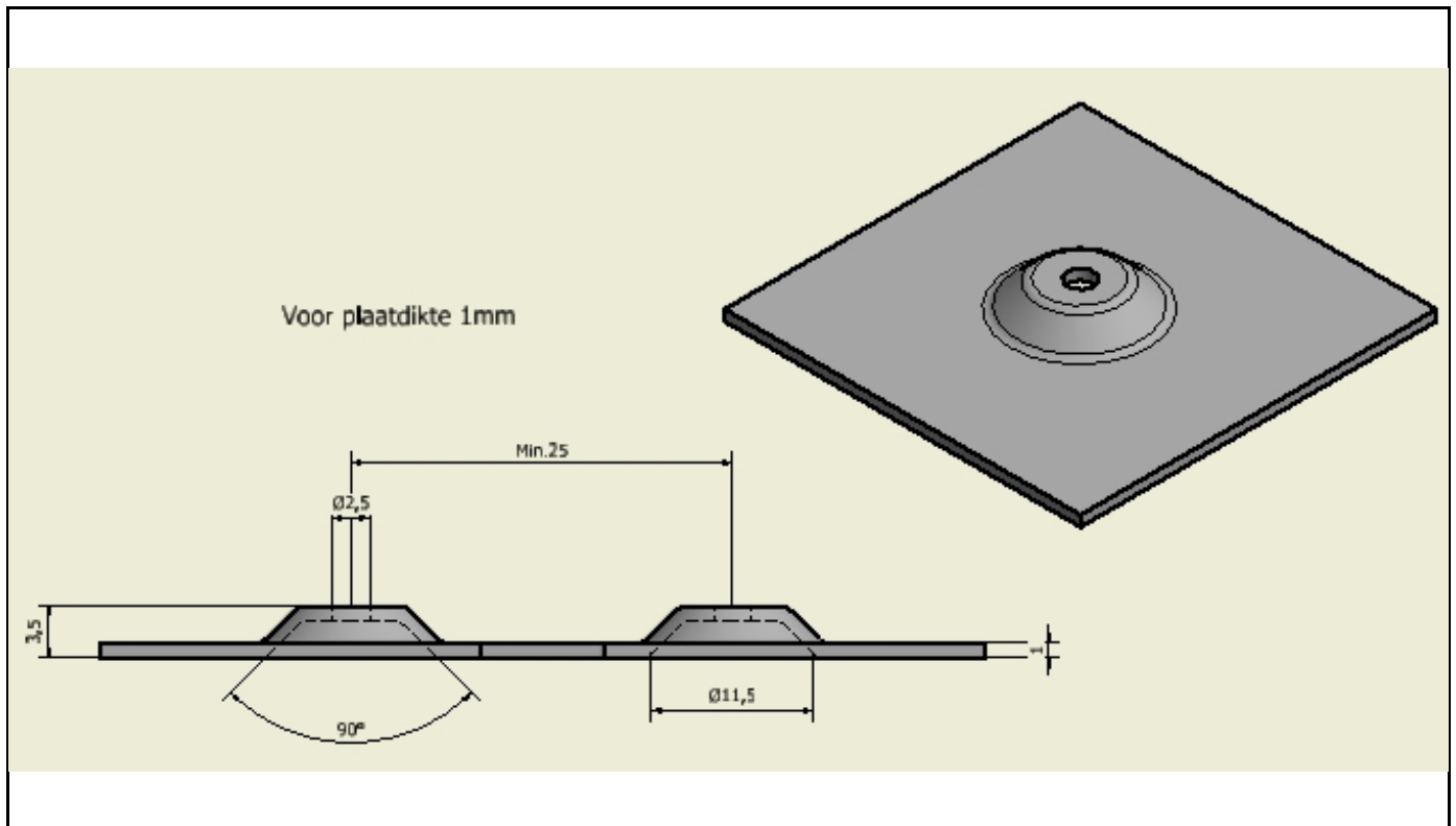
Cup forming tool upwards
