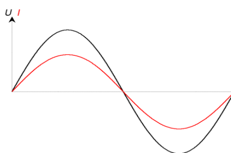
Typical input current shape when using a standard 6-pulse drive with RHF-Hybrid harmonic filter
