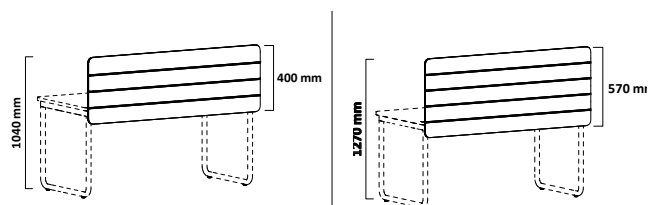
Play&Work 2.0 upper panel for U-LEG desk, upholstered with stitching, low
