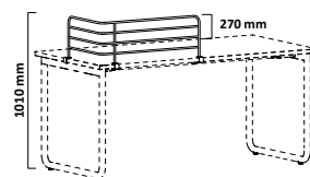
Play&amp;Work 2.0 upper panel, metal angular, low
