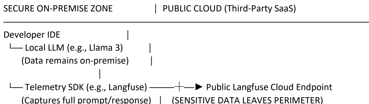
Figure 6: Insecure pattern — local LLM with public cloud telemetry (Section 4.6.1).
