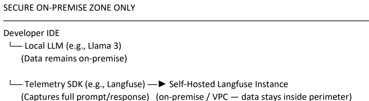
Figure 7: Secure pattern — local LLM with self-hosted telemetry (Section 4.6.1).
