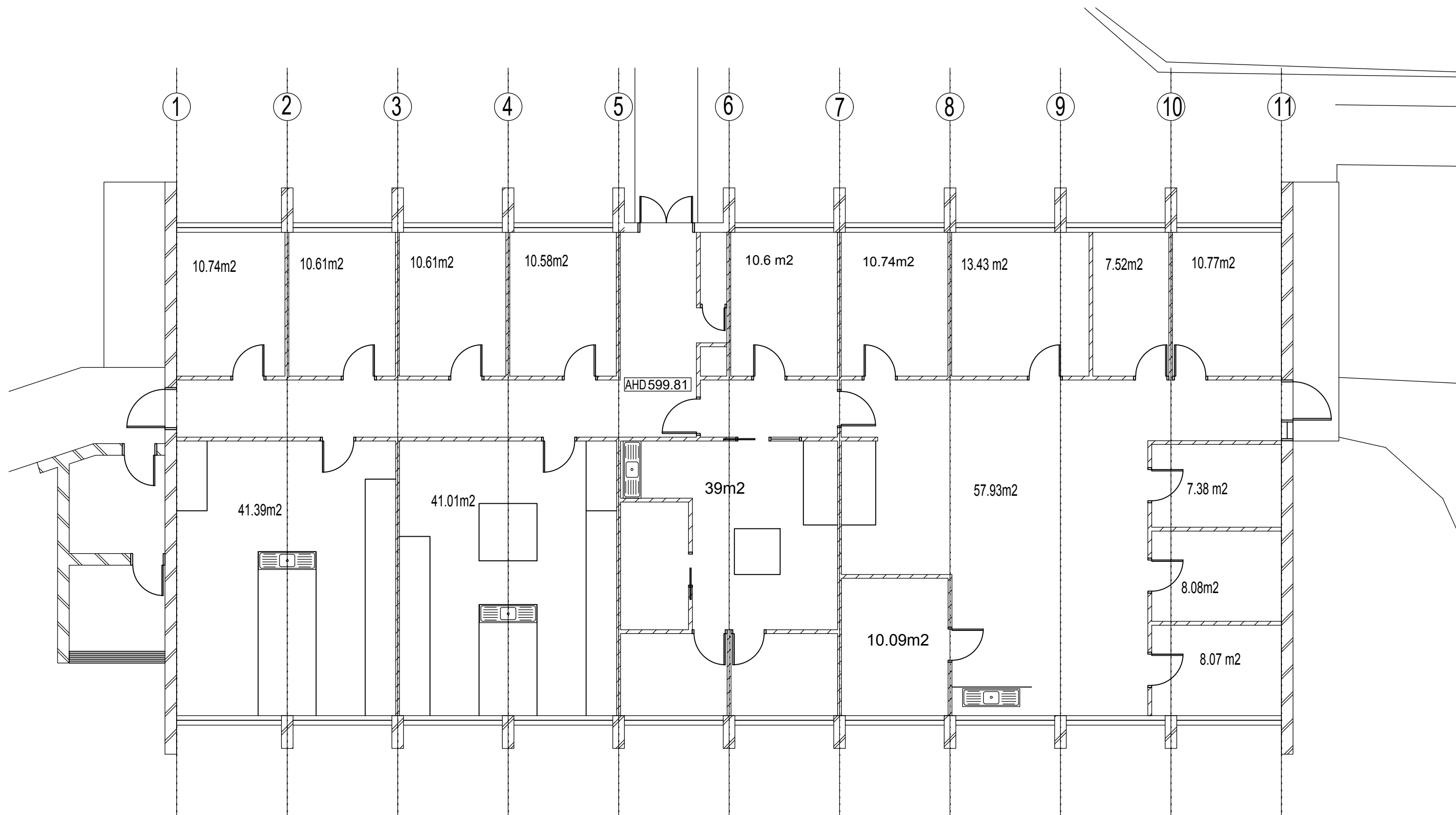
BUILDING 7 - LEVEL 1
