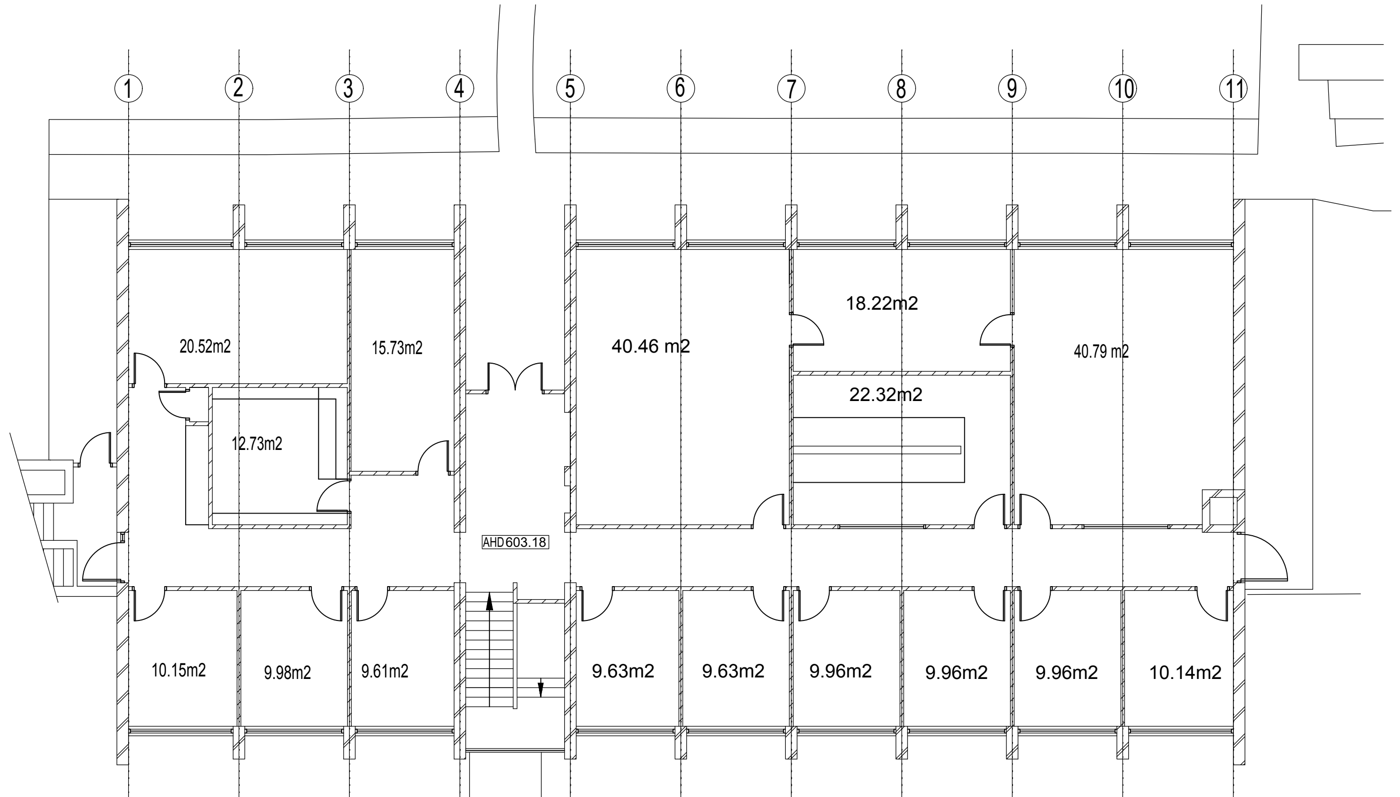
BUILDING 6 - LEVEL 2
