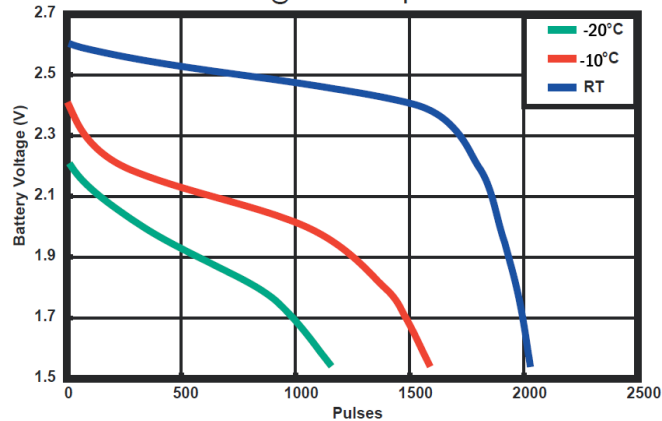
0.9 Amp, 3 sec on/27 sec off @ Various Temperatures
