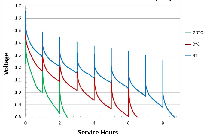
MX1500 AA - 3.9 Ohms at 1 Hour/Day
