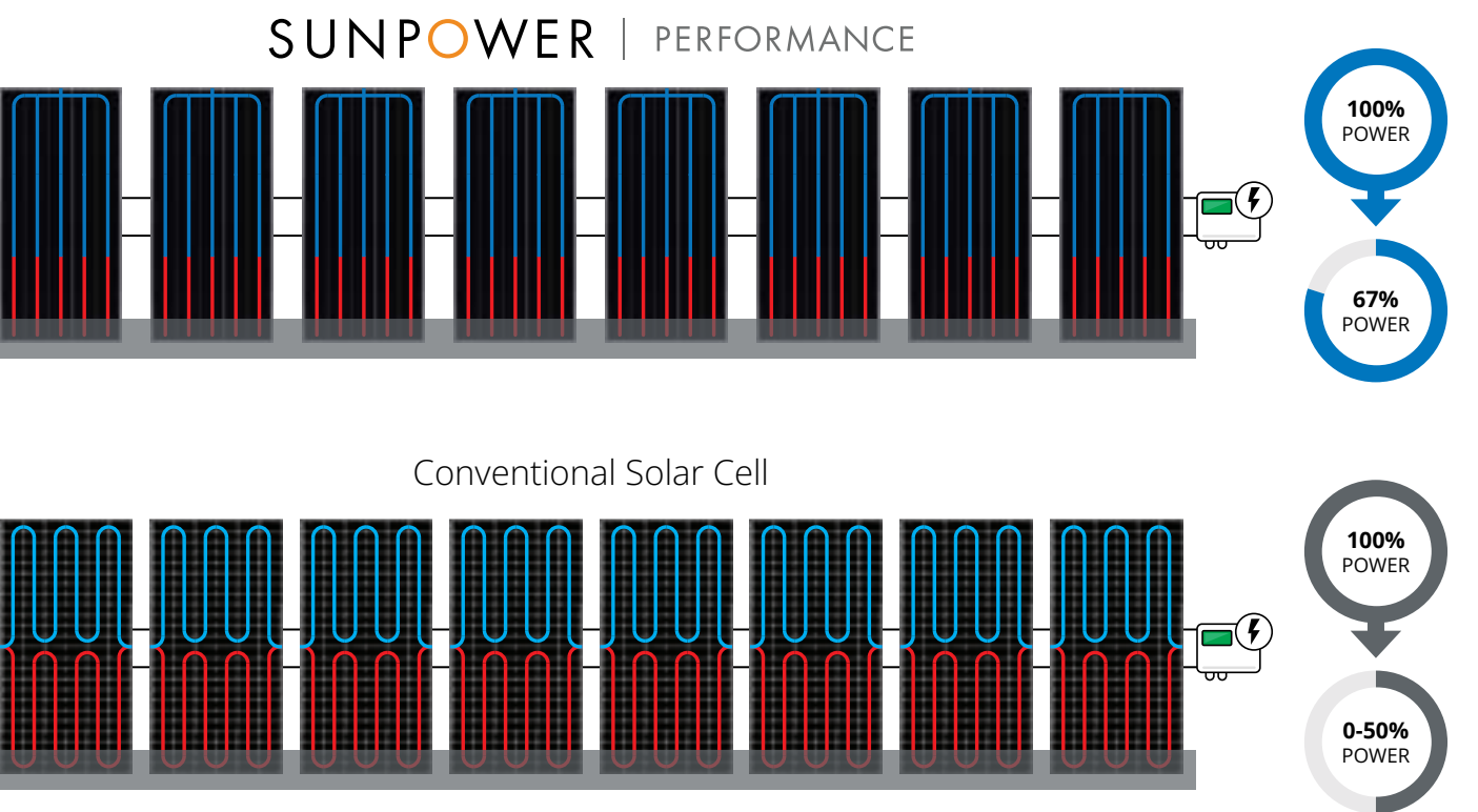
Figure 9: The Performance panel produces more energy than conventional panels when a consistent linear shadow is cast across the entire tracker row in portrait orientation.
