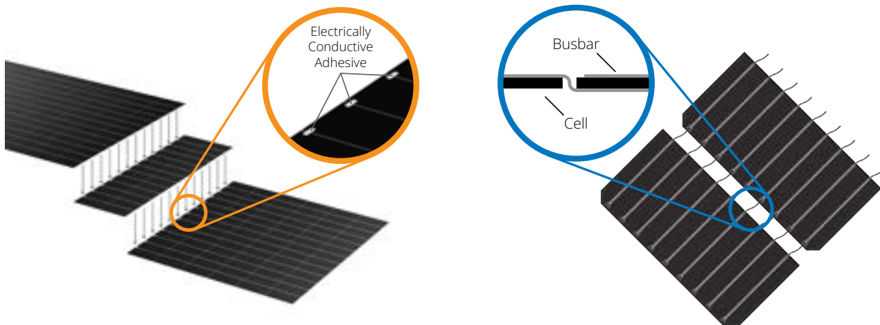
Figure 2: Performance panels eliminate the use of metallic wire cell connections—designing out one of the major failure modes of traditional cells.
