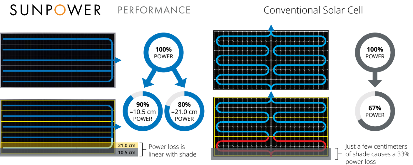
Figure 6: The parallel cell architecture of the Performance panel minimises power loss from shading and soiling in landscape orientation.
