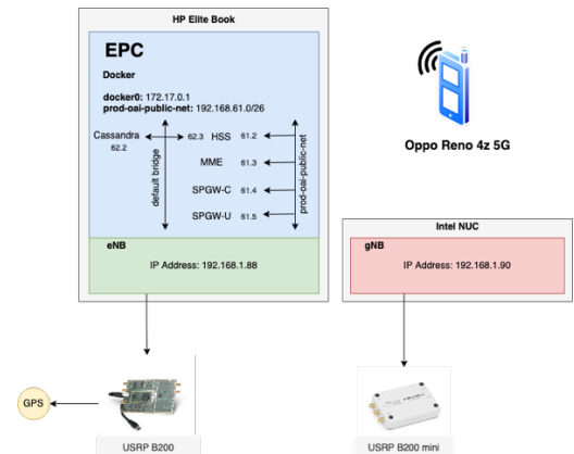
Figure 12: NSA Architecture
