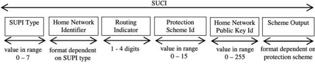
Figure 6: SUCI structure [7]
