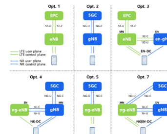
Figure 3: 5G deployment options [3]
