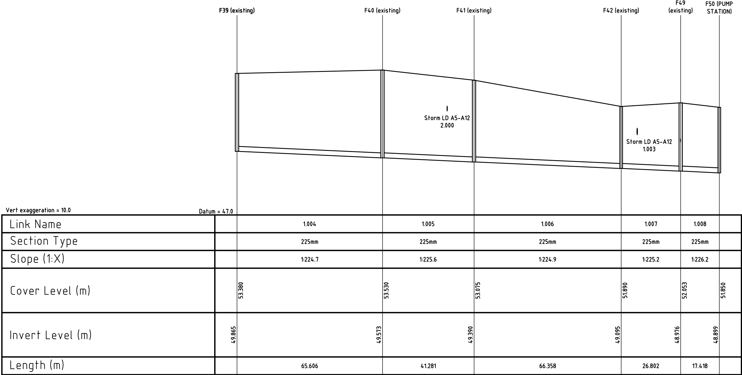
FOUL SEWER SECTIONS F39(EXISTING) – F50(EXISTING PUMP STATION) HORIZONTAL SCALE 1:1000 VERTICAL SCALE 1:100
