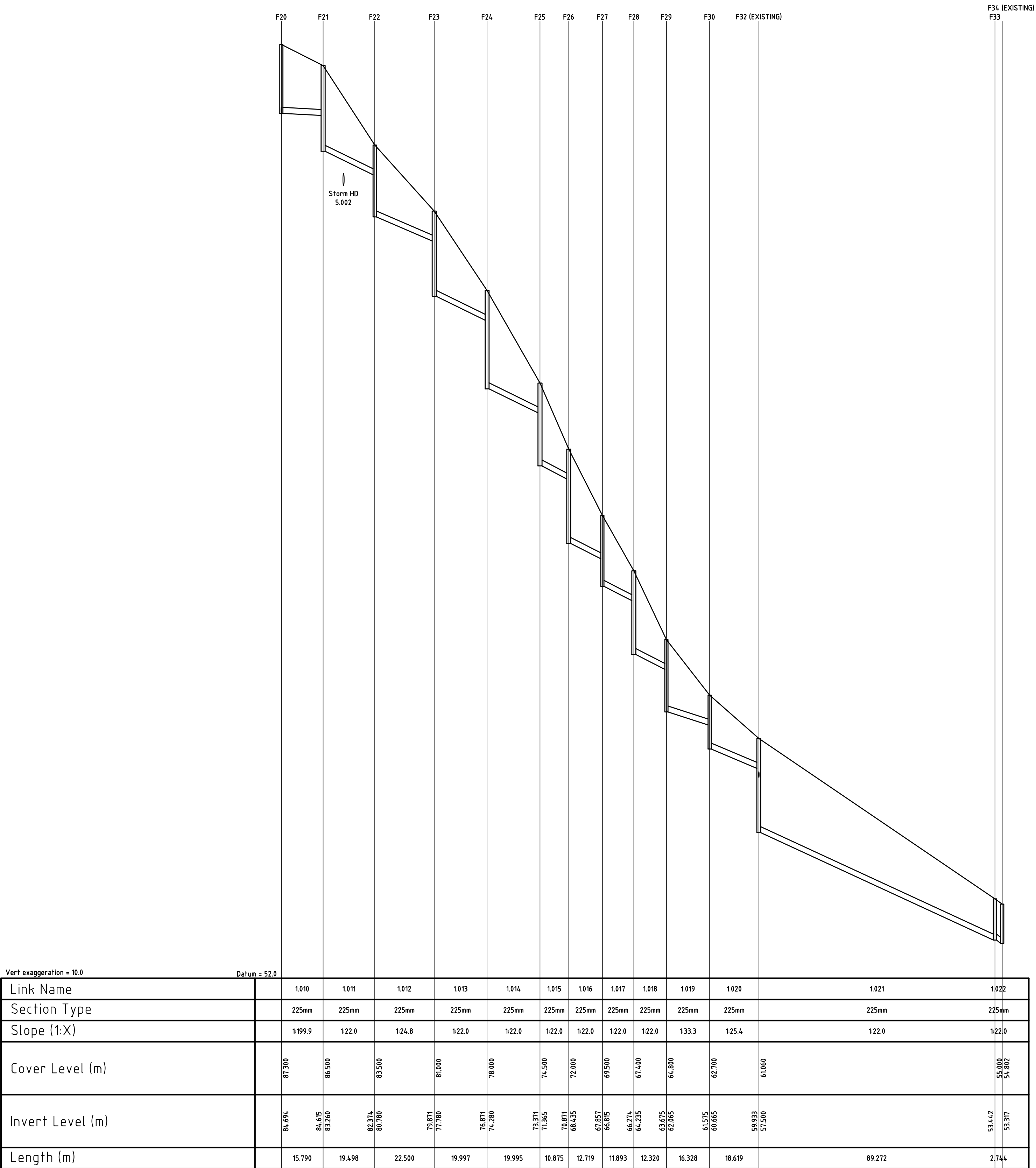
PROPOSED FOUL SEWER SECTIONS F20 – F34 (EXISTING) HORIZONTAL SCALE 1:1000 VERTICAL SCALE 1:100
