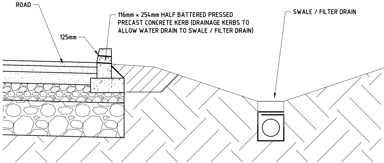
DRAINAGE KERB DETAIL (1:20)
