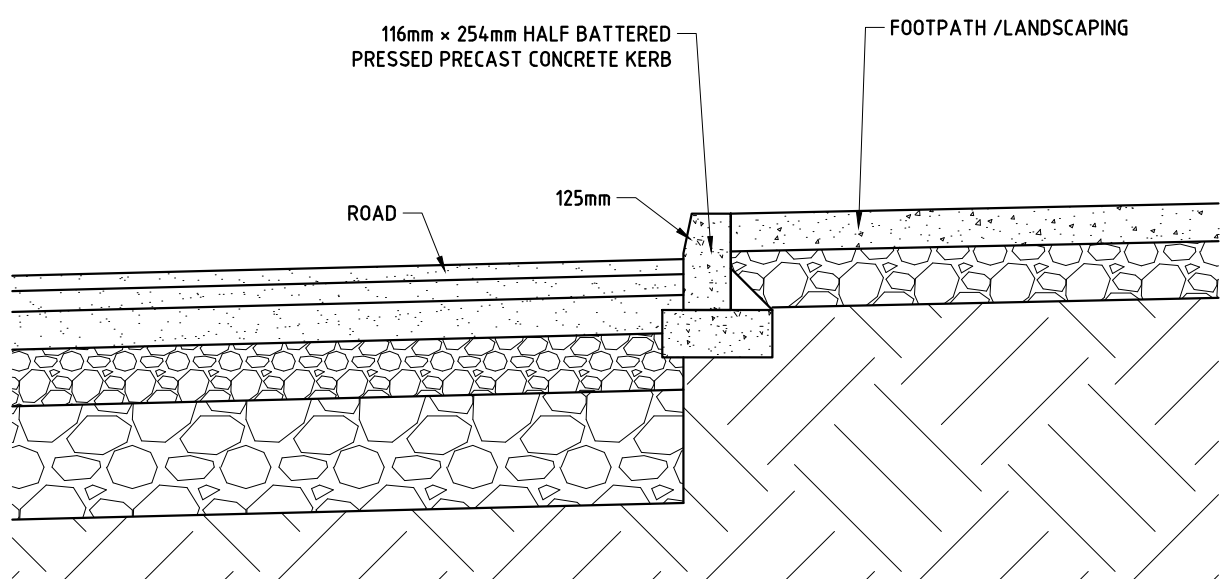
STANDARD KERB DETAIL (1:50)
