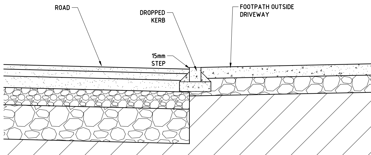
DROPPED KERB DETAIL AT DRIVEWAYS (1:50)
