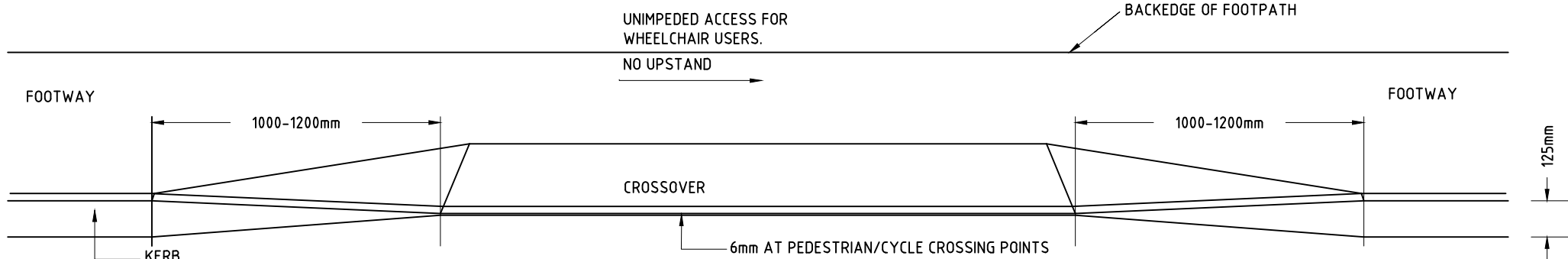
DROPPED KERB DETAIL AT PEDESTRIAN CROSSING POINT N.T.S
