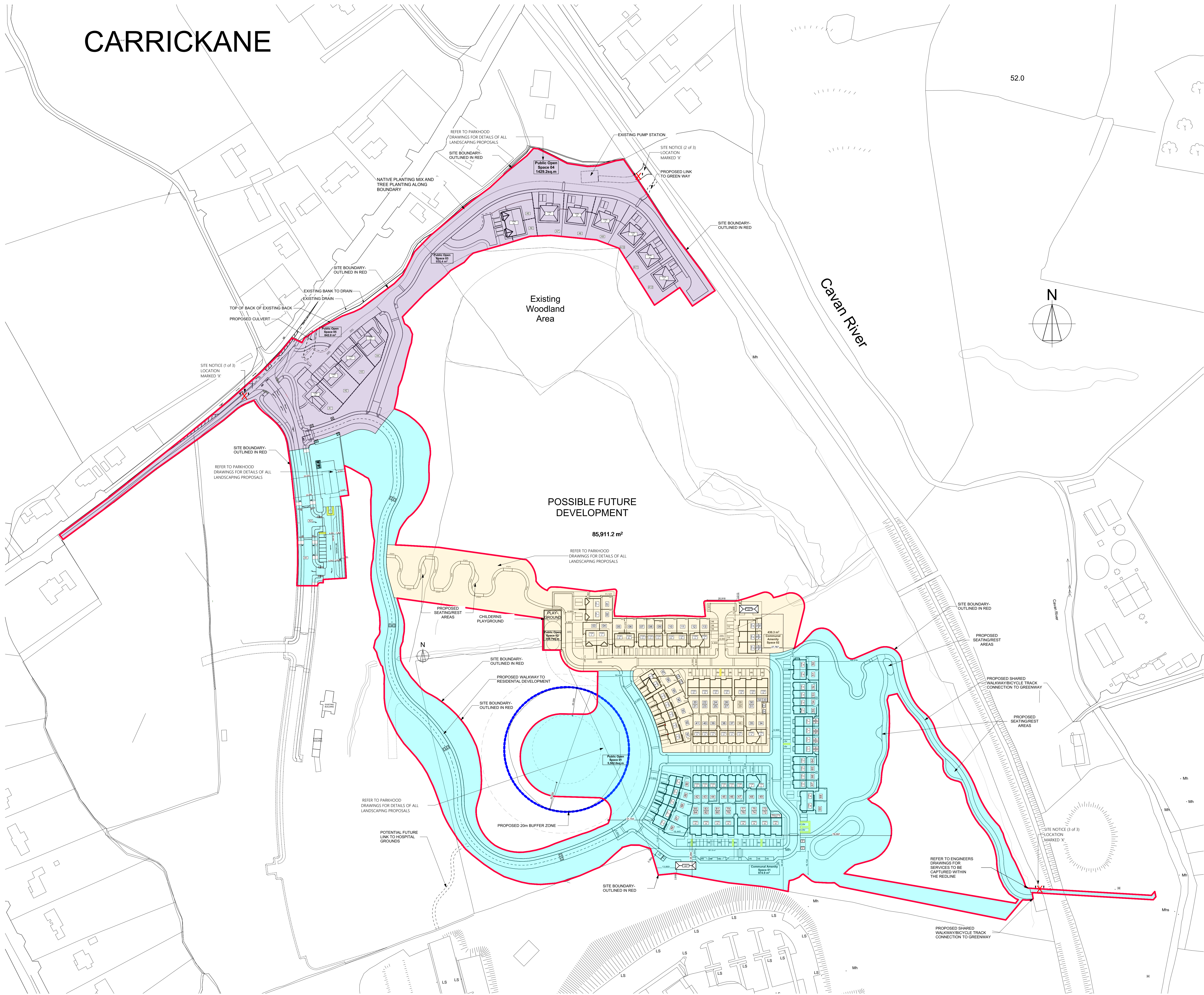
CONSTRUCTION PHASING MAP 1:1000
