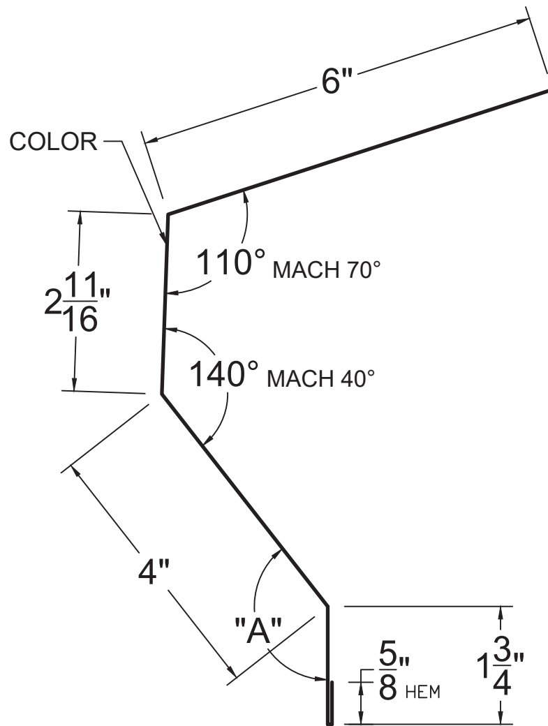
FINISHED ANGLE
