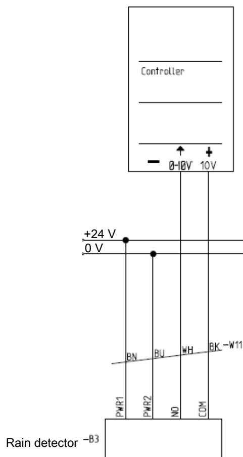
Figure 4: Example of connection to climate controller.
