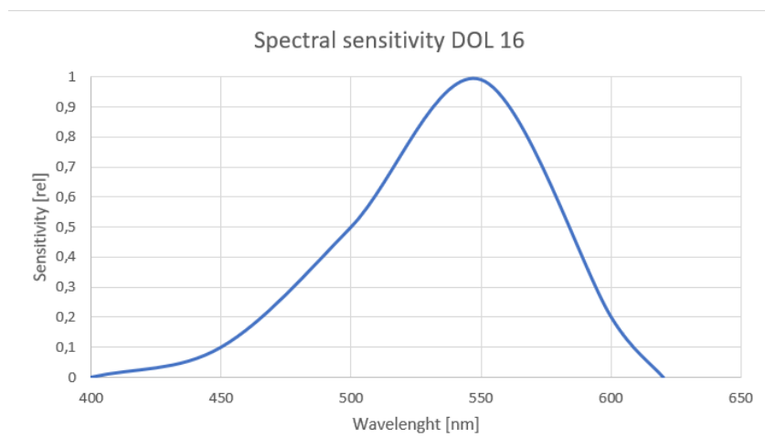
Figure 5: Spectral sensitivity.
