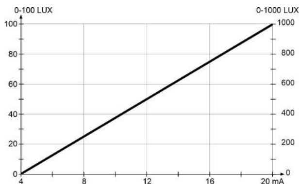
Figure 4: Function curve.
