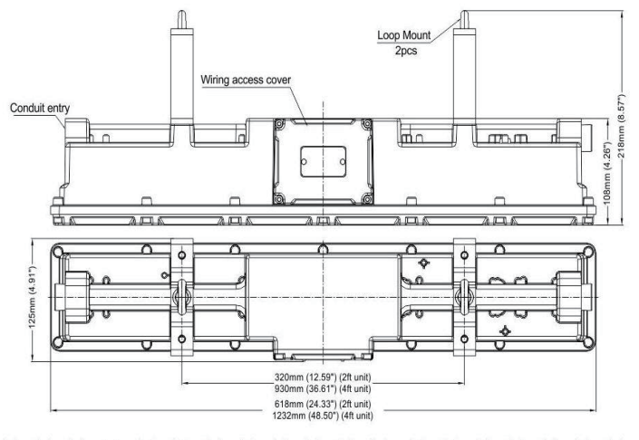
Loop Mount
