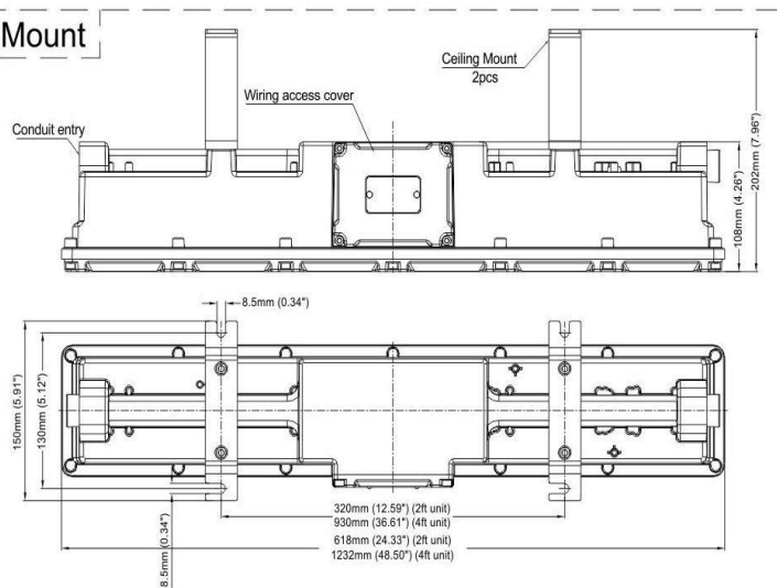
Trunnion Mount
