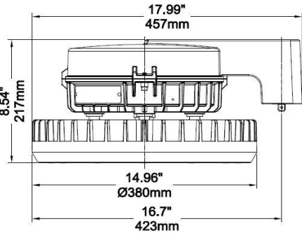
90° Stanchion Mount
