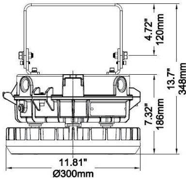
Trunnion Mount
