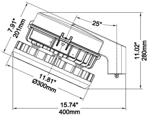
25° Stanchion Mount
