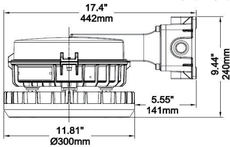
Wall Bracket
