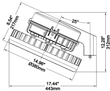
25° Stanchion Mount
