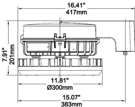
90° Stanchion Mount
