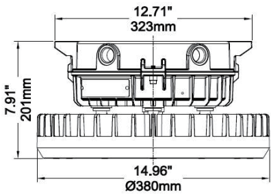
Celing Mount
