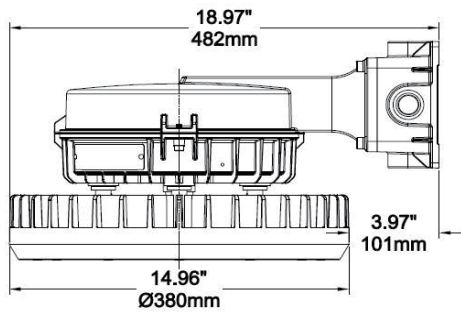
Wall Bracket
