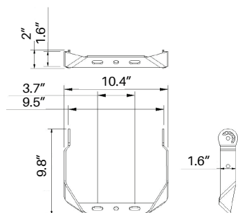
Single module Yoke Mount
