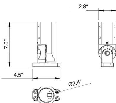
Ø2.4" Slipfitter (For single module)
