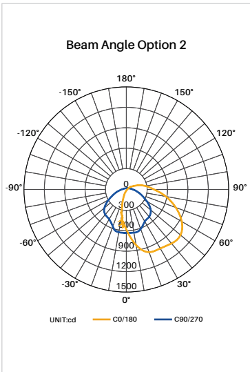
Frosted Lens
