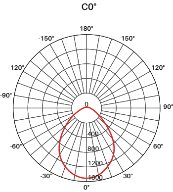
Distribution Curve C-plane — C0/180 — C90/270
