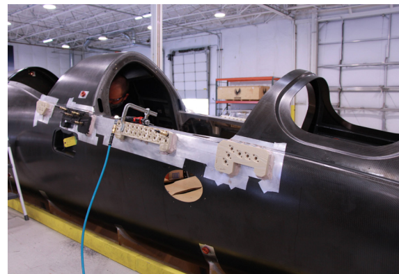
3D printed drill guides being used to drill fastener holes through a carbon fiber reinforced plastic (CFRP) and titanium stack-up in the XB-1 fuselage.
