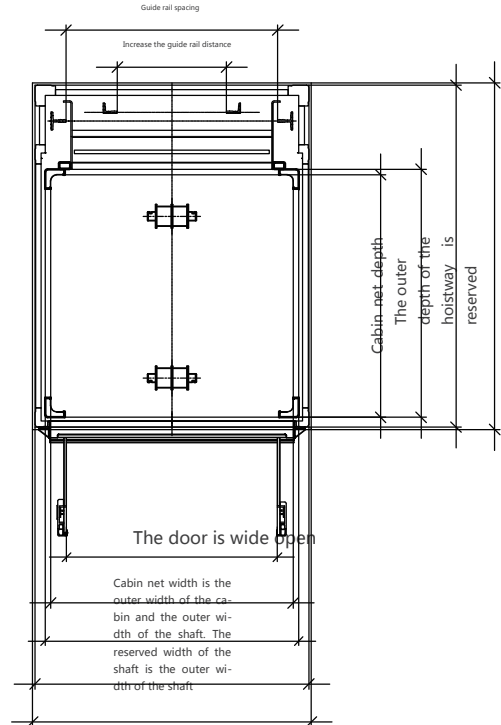
Cabin floor plan
