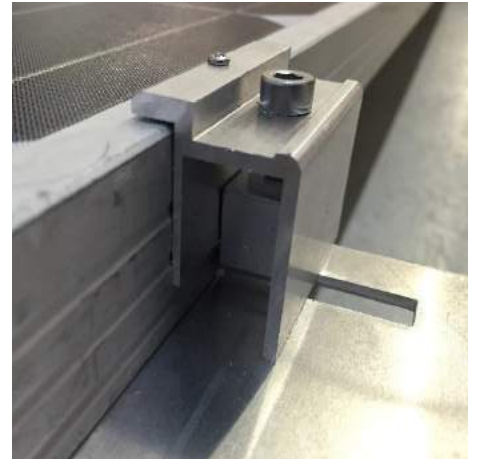
Fig. 9— Integrated End Clamp
