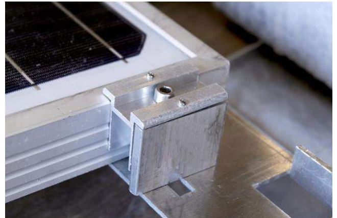
Fig. 11 – Insert End Block for End Clamps
