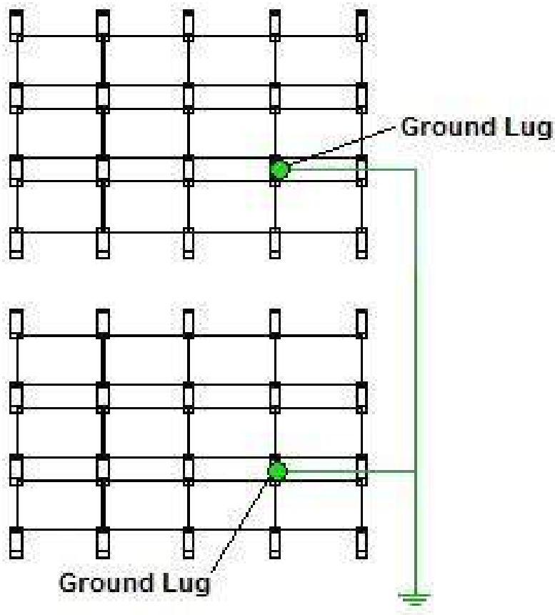
Figure 18 - Basic Wiring Diagram, Use as Example Only
