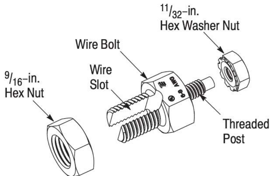
Figure 15 - Grounding Lug Schematic (Tyco model shown as an example)
