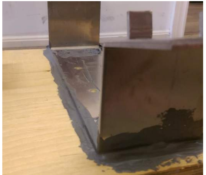
Figure 8 - Step 9: paint the H.E.R. UV resistant sealant around the perimeter of the AnchorRack
