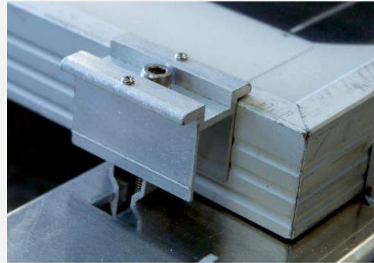
Figure 17 - Module Clamp
