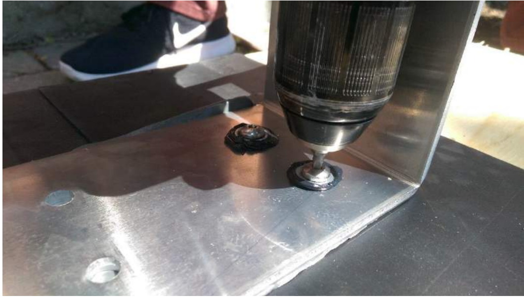
Figure 6 – Step 7: Screws and Washers drilled through applied LPS Sealant
