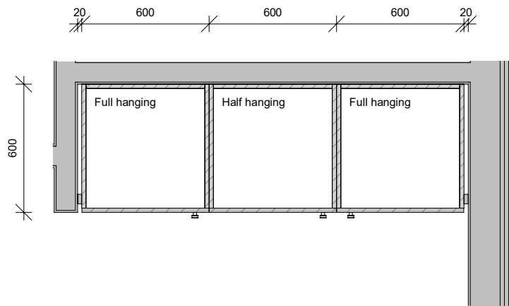
Typical Bedroom Plan
