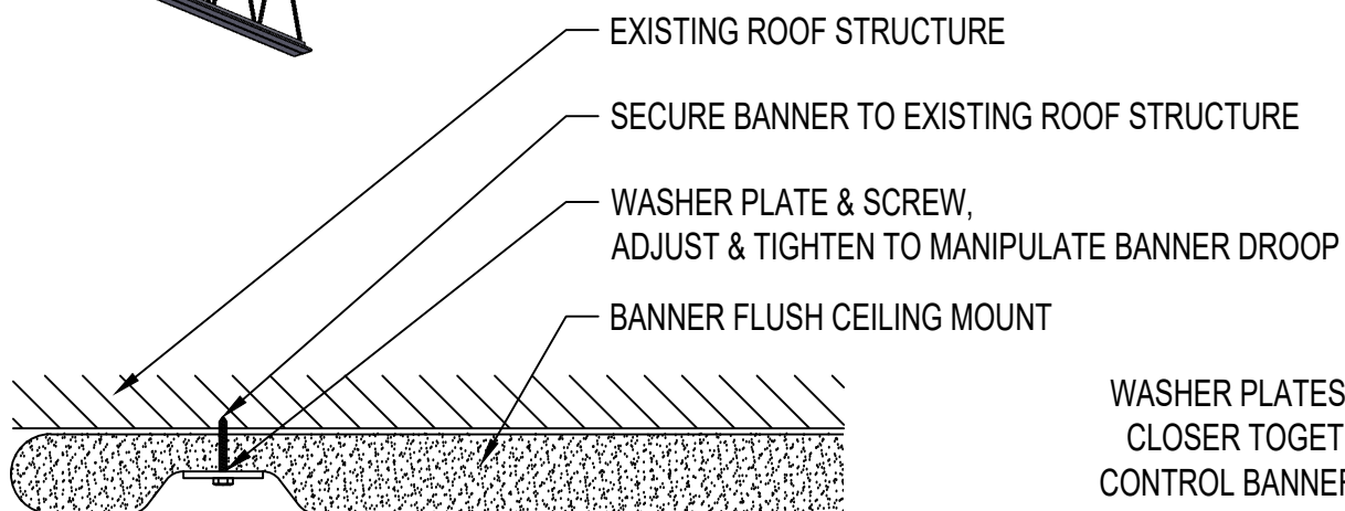
INSTALL DETAIL
