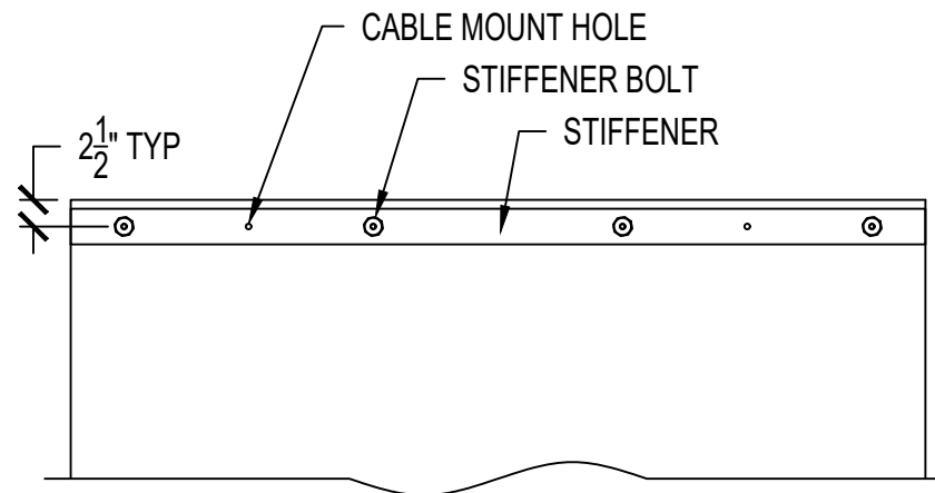
BANNER STIFFENER DETAIL
