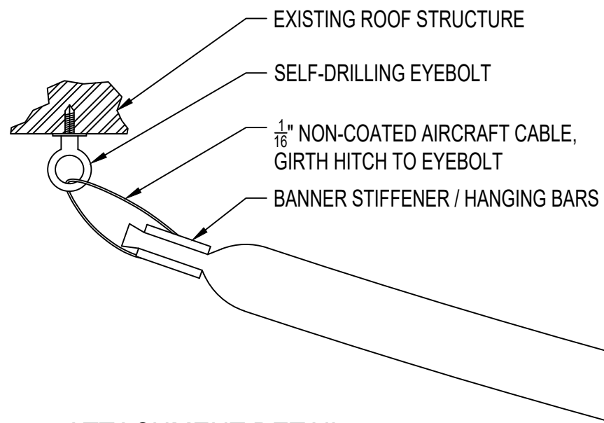
ATTACHMENT DETAIL
