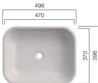
VDS 470.370.R80
