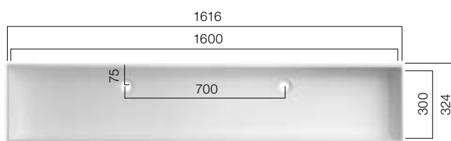
VDC 1600_300
