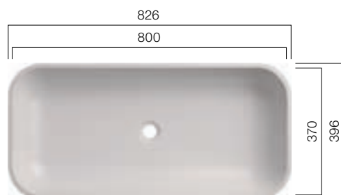
VDS 800.370.R80
