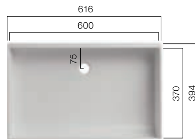
VDC 600
