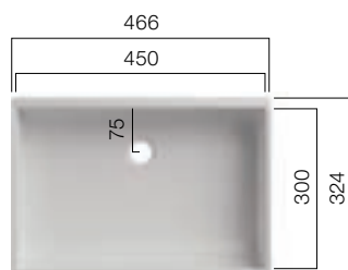
VDC 450.300
