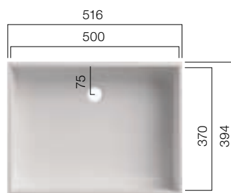
VDC 500
