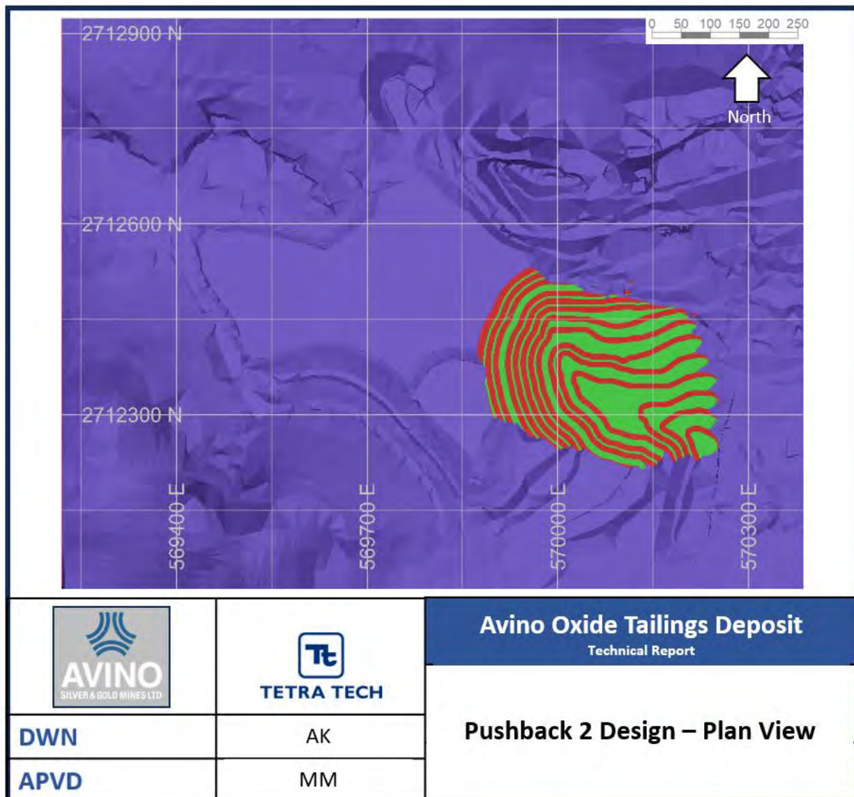
Figure 15-13: Pushback 2 Design
