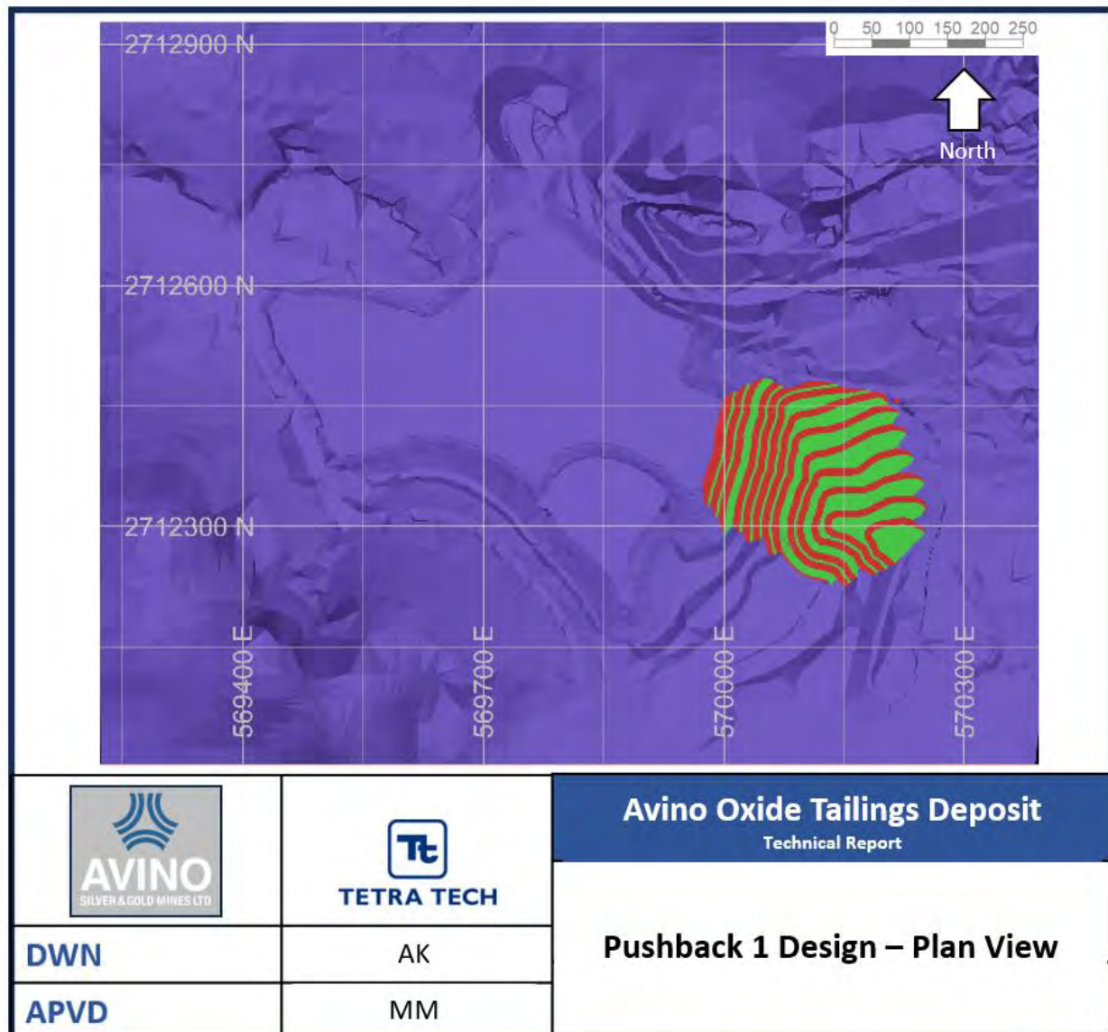
Figure 15-12: Pushback 1 Design
