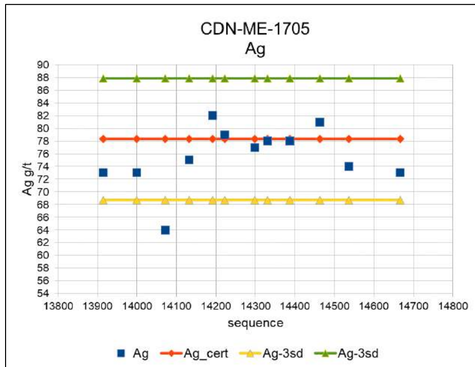
Figure 11-14: Reference Material CDN-ME-1705 Ag Performance
