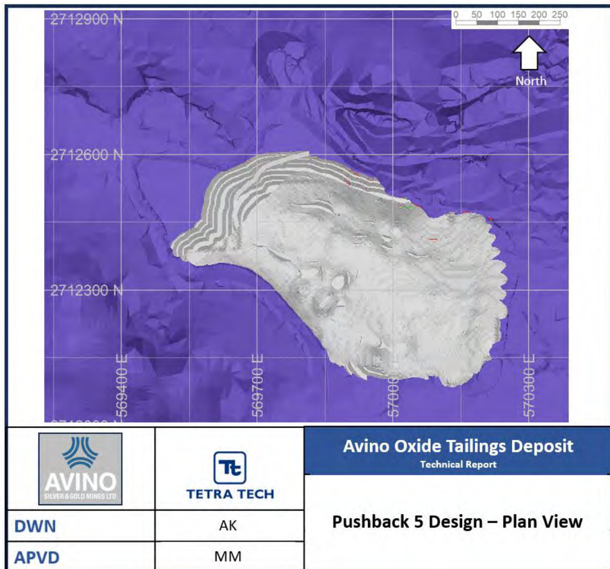
Figure 15-16: Pushback 5 Design
