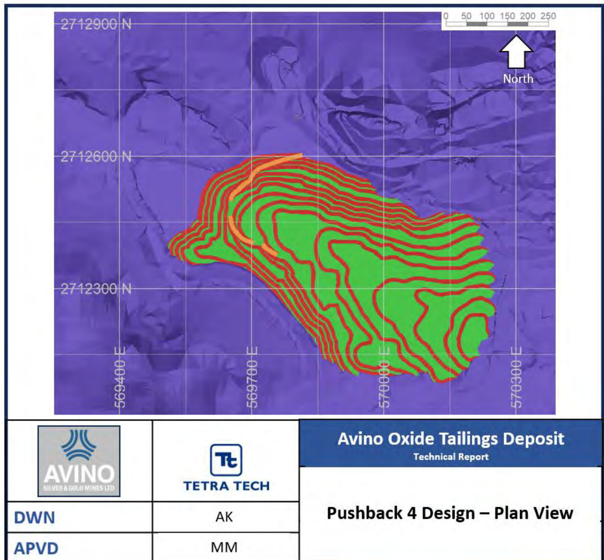
Figure 15-15: Pushback 4 Design
