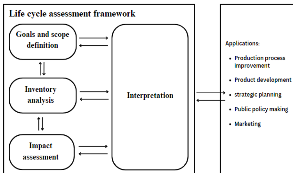
Figure 1 LCA Framework
