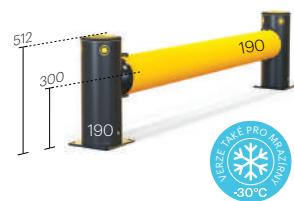
iFlex Single Traffic Barrier **
