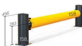
eFlex Single Traffic Barrier **
