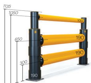
Atlas Double Traffic Barrier+ **
