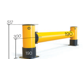
iFlex Single Rackend Barrier **
