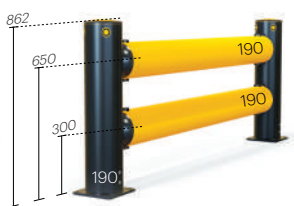
iFlex Double Traffic Barrier **
