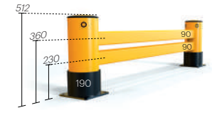
eFlex Double Rackend Barrier **
