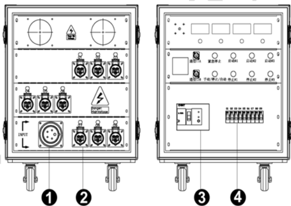
Figure 2-8 Internal Structure of Distribution Box
