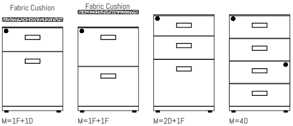
Metal Pedestals With Recessed Handles
